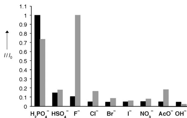
Figure 2. Normalized fluorescence response I / I 0 of polymer 1a (black bars) and model compound 2 (gray bars) to anions \text{X}^- ( n\text{Bu}_4\text{N}^+\text{X}^- , 10% \text{H}_2\text{O} /NMP solvent; anion concentration 140 μM for 1a and 1200 μM for 2 , respectively).
